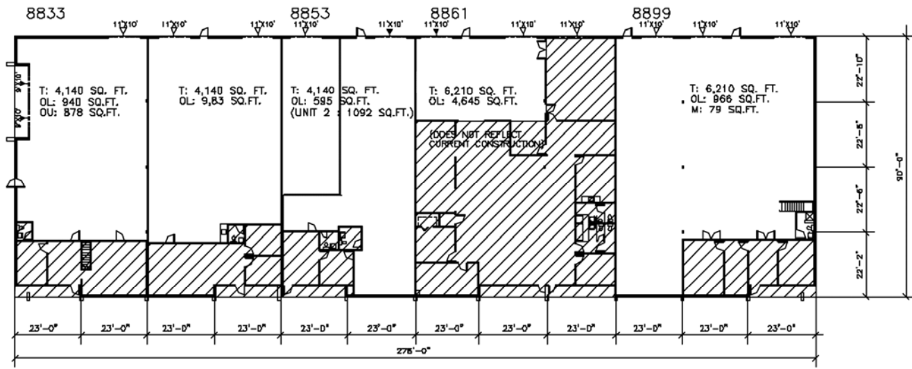
CLACKAMAS BUSINESS CENTER - BUILDING "E" - 24,840 SQ.FT. NOT TO SCALE 0 4 8 12 20 36 FT
