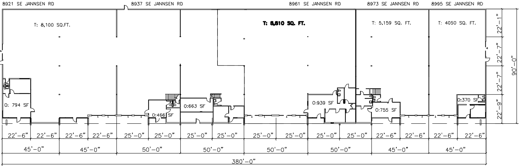
FIRST FLOOR PLAN - BUILDING D 34,200 SQ. FT. NOT TO SCALE
